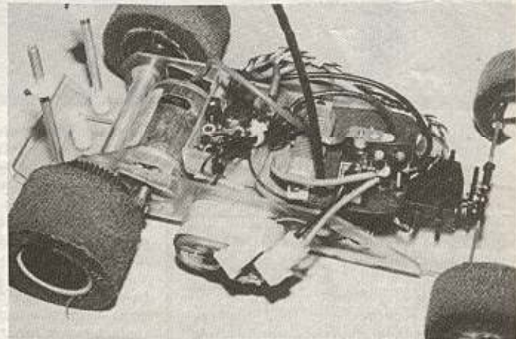
Above left: resistor speed control plus micro-switch for reverse operation. Futaba steering servo is fitted with Schumacher servo saver. Above: torque tube and motor mount, a Schumacher differential is fitted in this instance. Below left: underside view showing battery retention method and chassis fretting-out. Below: completed chassis ready to roll. Note receiver in Parma lightweight case.
